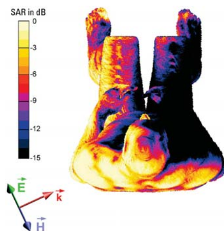
Figure 2. SAR distribution on the surface of a male (80 kg) in a sitting position (top view): 0 dB corresponds to 0.05 \text{ W/kg} for an E-field strength of 1 V/m. The orientation of the E-field ( \vec{E} ), the magnetic field ( \vec{H} ), and the propagation direction ( \vec{k} ) of the EMF are indicated.
